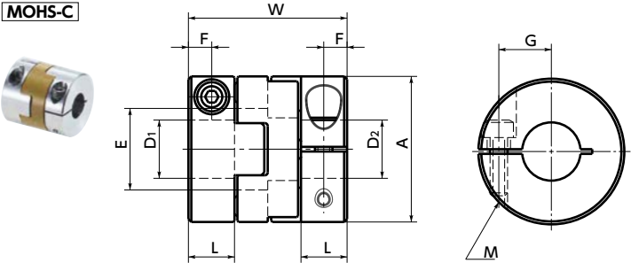
MOHS-C
