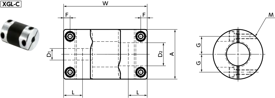
XGL-C
