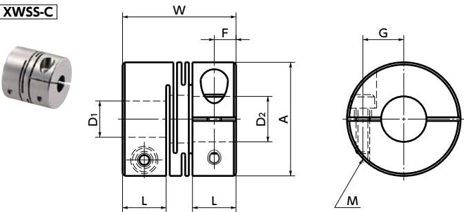
XWSS-C
