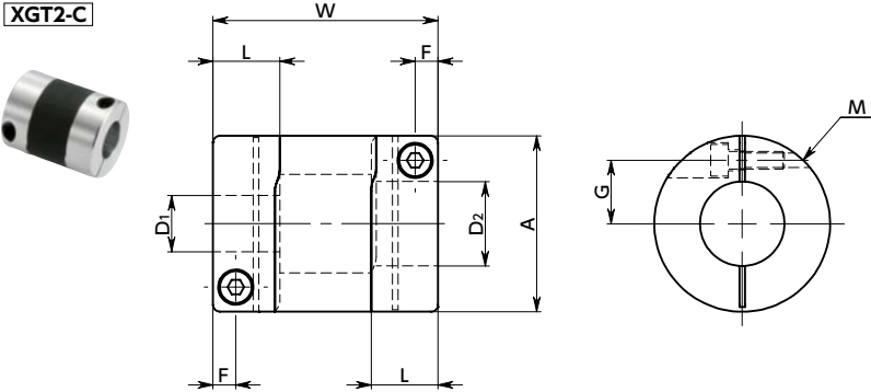
XGT2-C
