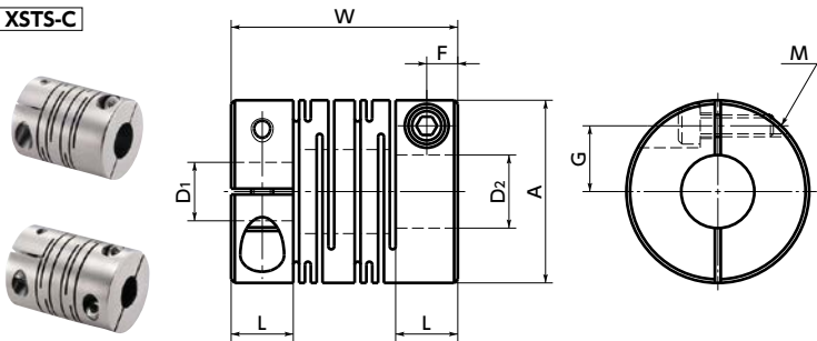
XSTS-C
